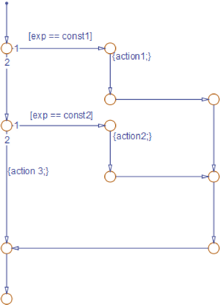
switch with two cases and default
